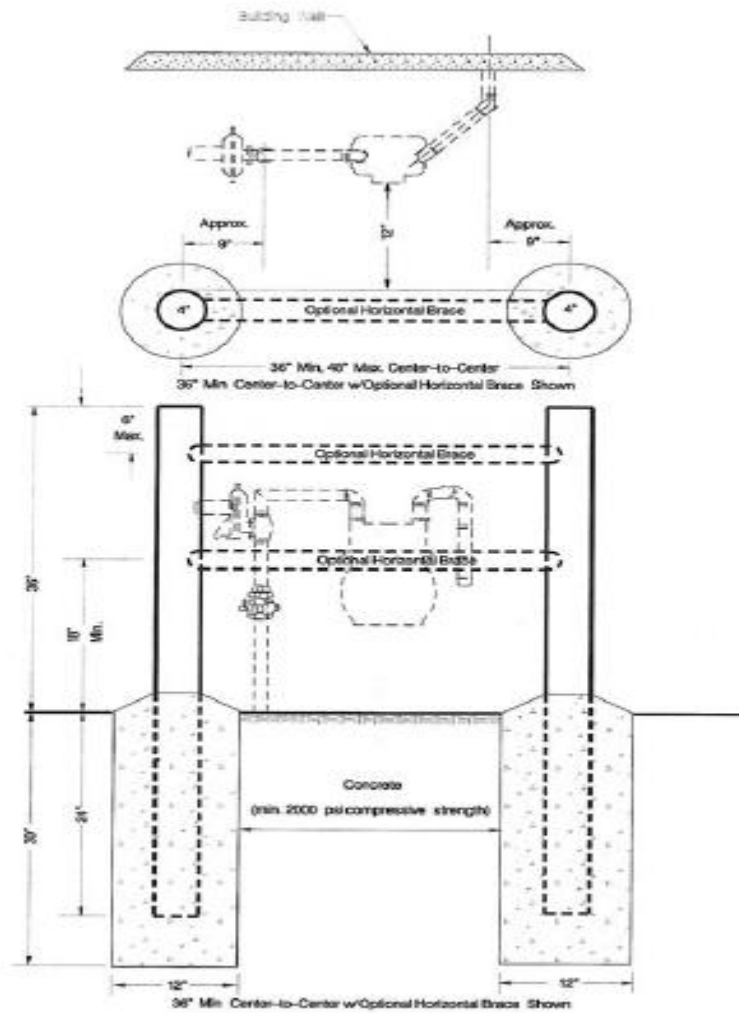
Illustration 4.0 – Typical 4 Inch Gas Meter Guard
