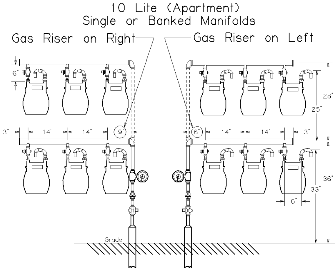
Illustration 7.0 – Typical Multi-Meter Installations and Dimensions
