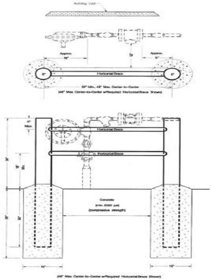
Illustration 5.0 – Typical 6 Inch Gas Meter Guard
