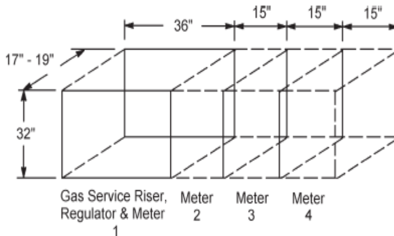
Illustration 6.0 – Cabinet Dimensions for Multiple Residential Meters
