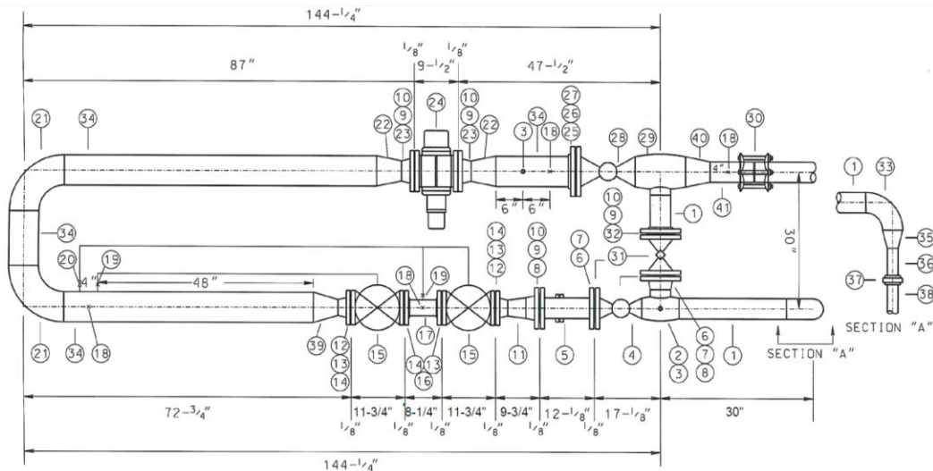
Diagram of typical 16M Rotary Industrial Meter Set
