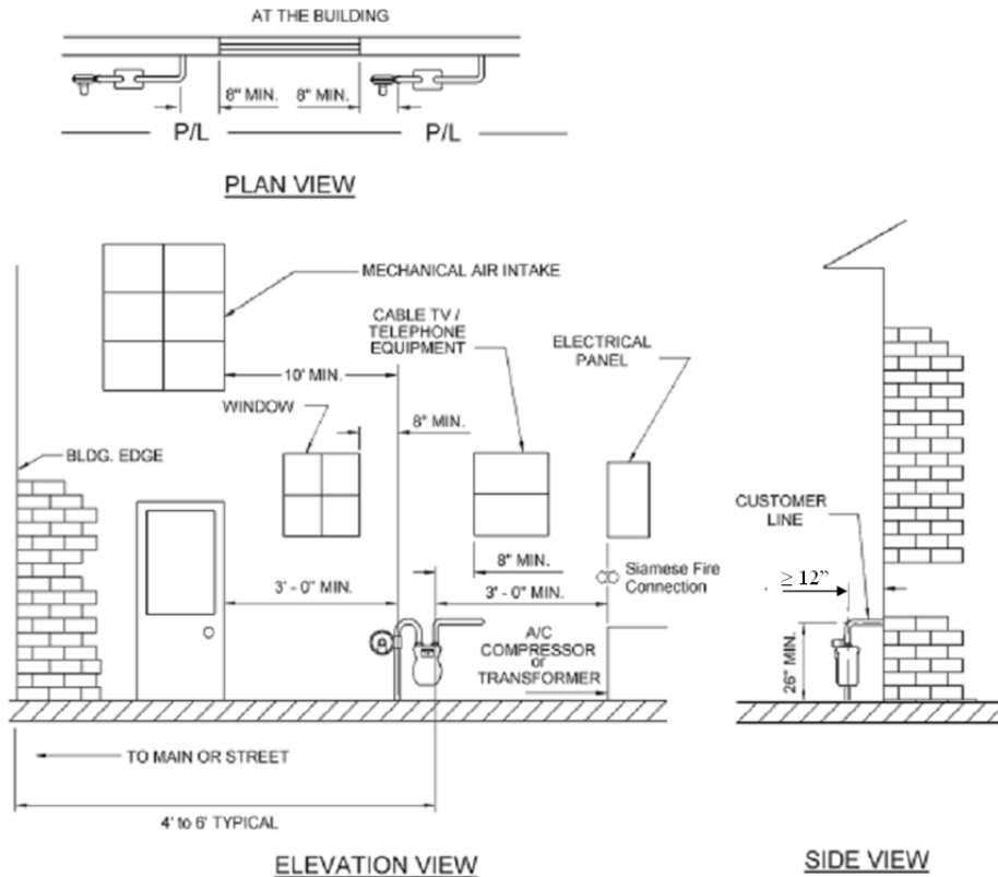
Illustration 3.0 – Typical Meter Set Clearances
