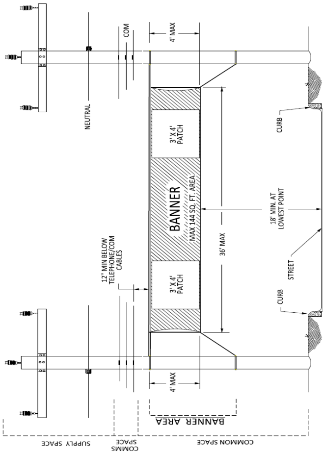
PROFILE DRAWING NOT TO SCALE
